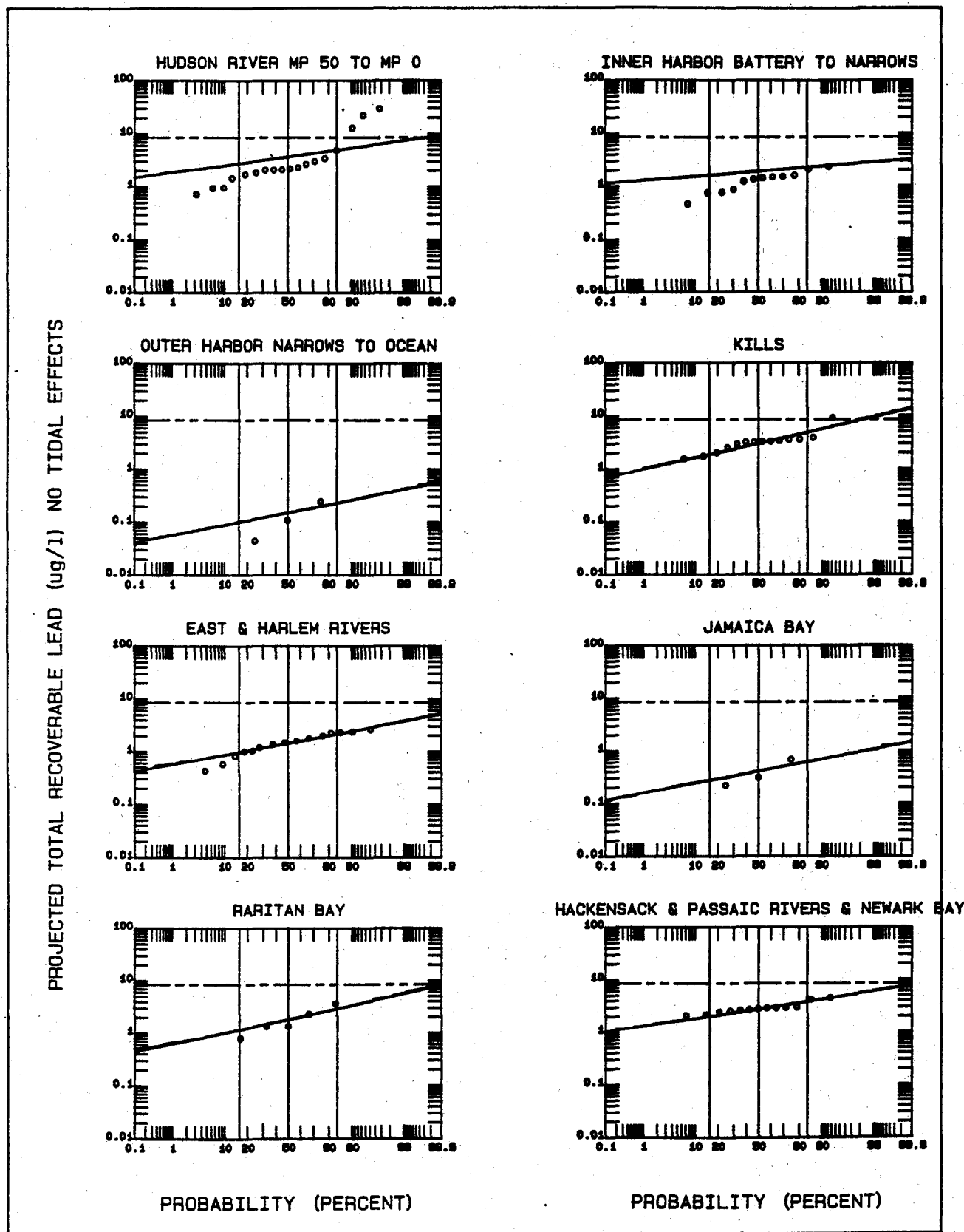
Figure 4. Log Probability Distributions of Total Recoverable Lead for a Projected Non-Tidal Condition.
