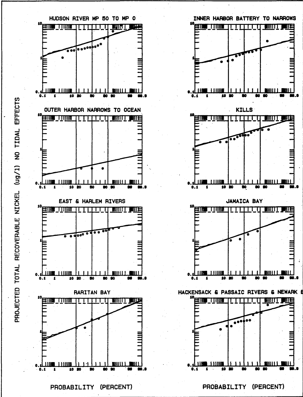
Figure 3. Log Probability Distributions of Total Recoverable Nickel for a Projected Non-Tidal Condition.
